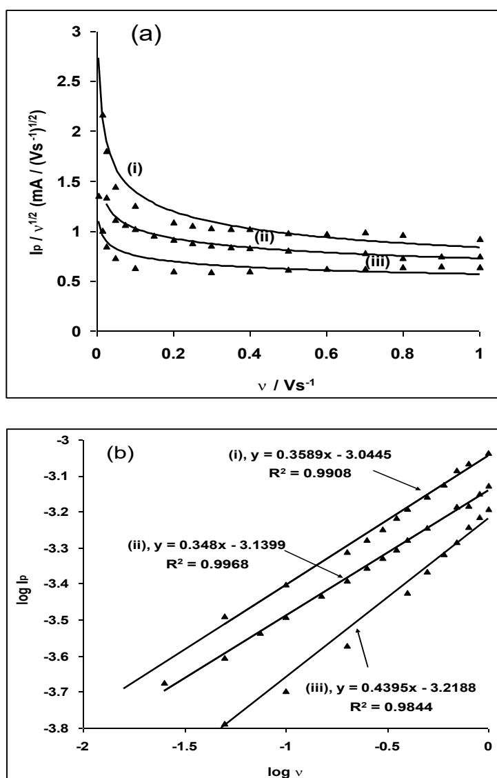
Figure 7. (a) Current function plots of ( I_p/v^{1/2} vs v ) for (i) \text{IO}_3^- , (ii) \text{IO}_4^- and (iii) \text{SO}_3^{2-} . (b) Plots of \log I_p vs \log v for (i) \text{IO}_3^- , (ii) \text{IO}_4^- and (iii) \text{SO}_3^{2-} .
