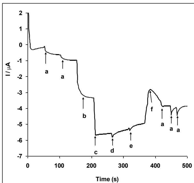
Figure 9. Typical Amperometric response of Pt-MWCNT-PB electrode for (a) 1.8 mM \text{IO}_3^- and in the presence of 1.0 mM of various interference species (b) nitric oxide ( \text{NO} ), (c) nitrite ( \text{NO}_2^- ), (d) bromate ( \text{BrO}_3^- ), (e) chlorate ( \text{ClO}_3^- ) and (f) sulphite ( \text{SO}_3^{2-} ). A potential of 0.32 V and PBS of pH 2 was used.
