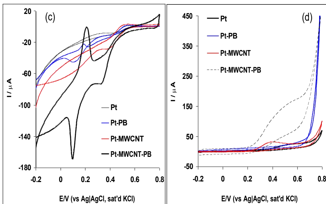
Figure 5. (a) Comparative current response of the modified Pt-MWCNT-PB electrode in pH 2.0 PBS alone, and pH 2.0 PBS + 8 mM IO_3^- . (b), (c) and (d) are the comparative cyclic voltammograms showing the current response of Pt, Pt-PB, Pt-MWCNT and Pt-MWCNT-PB modified electrodes in 8 mM IO_3^- in pH 2.0 PBS, 8 mM IO_4^- in pH 2.0 PBS and 8 mM SO_3^{2-} in 0.1 M NaOH respectively (Scan rate: 25 mVs -1 ).
